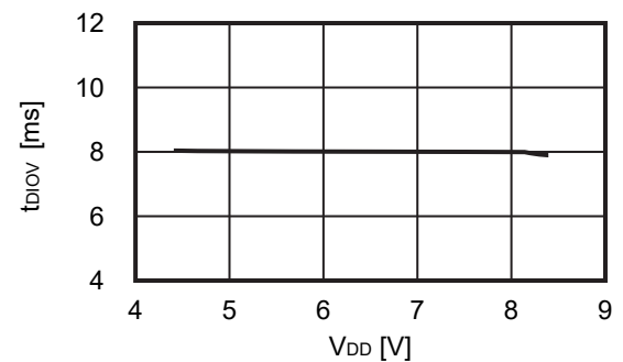
2.8 t_{DIOV} - V_{DD}
