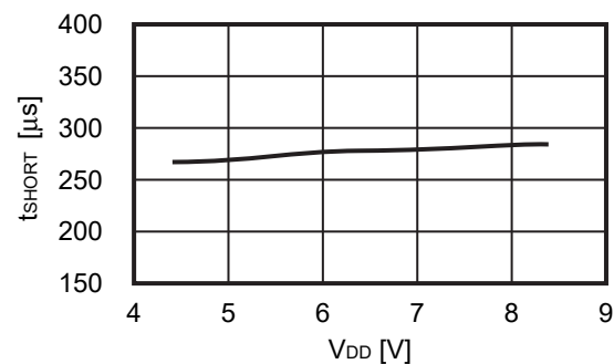
2.14 t_{SHORT} - V_{DD}
