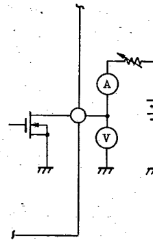
TEST CIRCUIT
